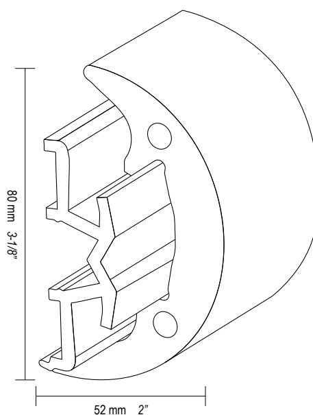
RADIAL 80
